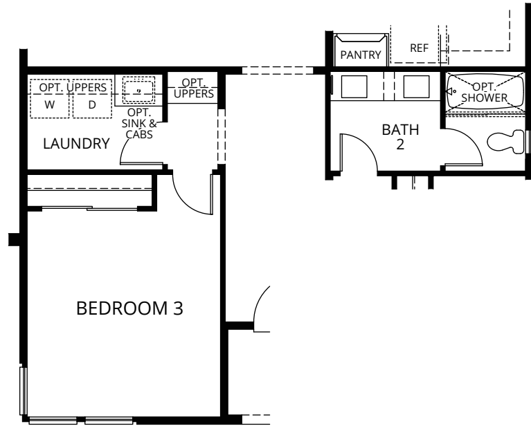
STANDARD BEDROOM 3
