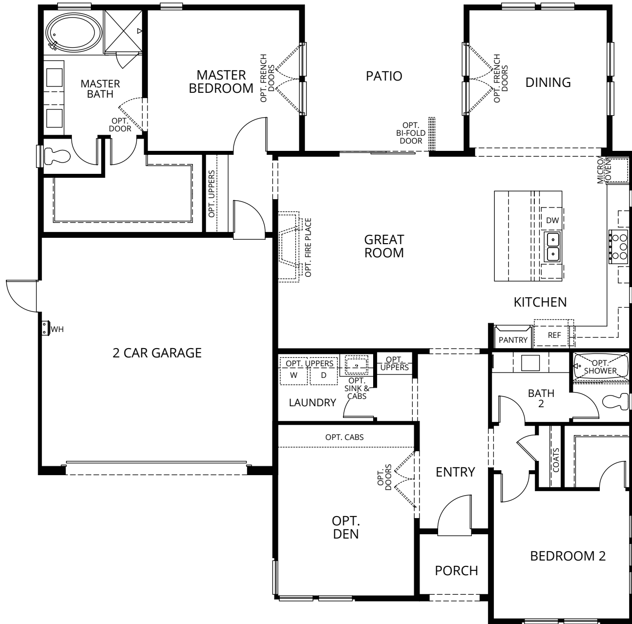
FLOOR PLAN
